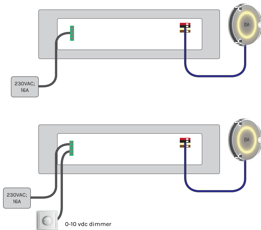
Overview - Combination of MONO SubAqua LED underwater lights and Power Supply Units
