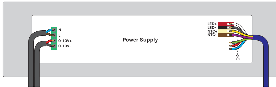
Connections to the Power Supply Unit of the EVA B2 LED underwater light (incl. dimmer)
