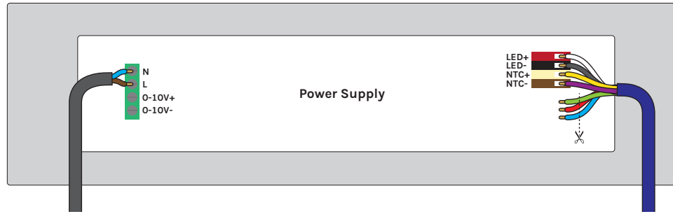
Connections to the Power Supply Unit of the EVA B2 LED underwater light (excl. dimmer)
